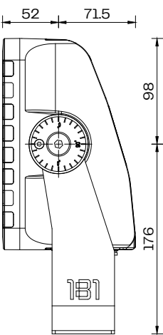
Beam F120 Side Scale 1:5
