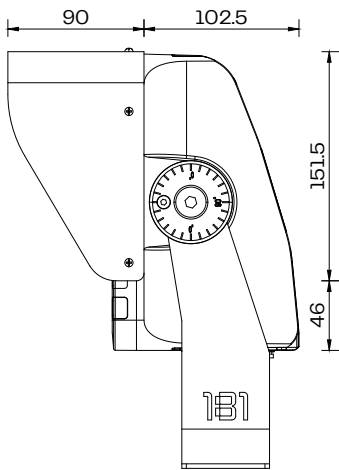
Beam F120 with Half Glare Shield Side Scale 1:5
