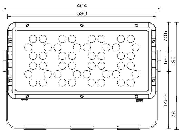
Beam F120 Front Scale 1:5
