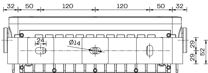
Beam F120 Bottom Scale 1:5
