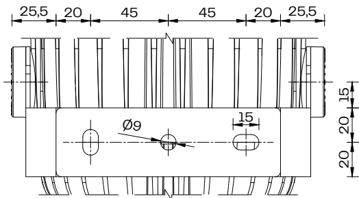
Beam F36 Bottom Scale 1:3
