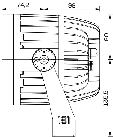
Beam F36 Side Scale 1:4
