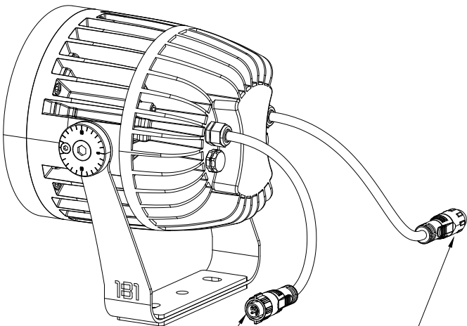
Input Connector M16 5Pin Male
