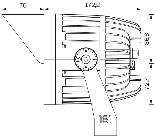
Beam F36 with Half Glare Shield Side Scale 1:4
