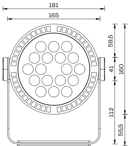
Beam F36 Front Scale 1:4
