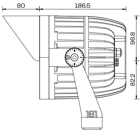
Beam F54 with Half Glare Shield Side Scale 1:5
