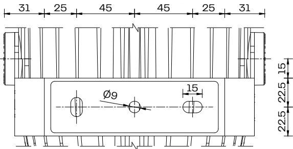
Beam F54 Bottom Scale 1:3
