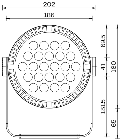
Beam F54 Front Scale 1:5
