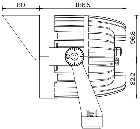
Beam F54 with Half Glare Shield Side Scale 1:5
