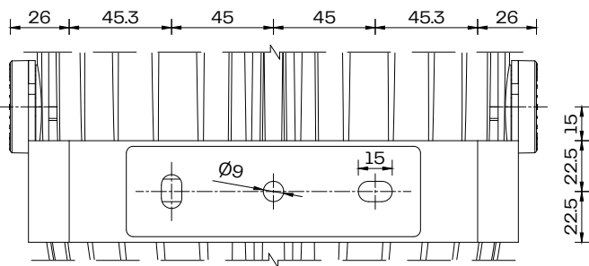
Beam F72 Bottom Scale 1:3
