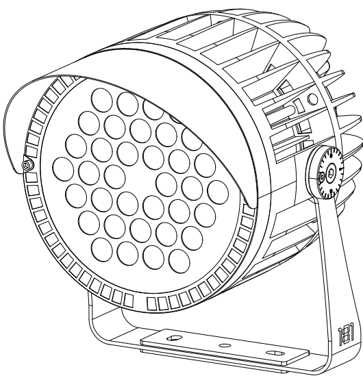
Beam F72 with Half Glare Shield
