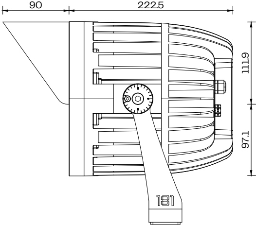
Beam F72 with Half Glare Shield Side Scale 1:5
