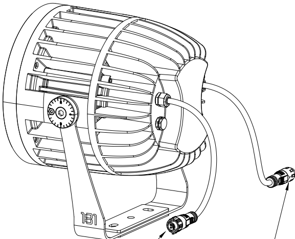
Input Connector M16 5Pin Male
