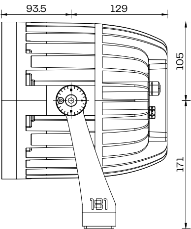
Beam F72 Side Scale 1:5
