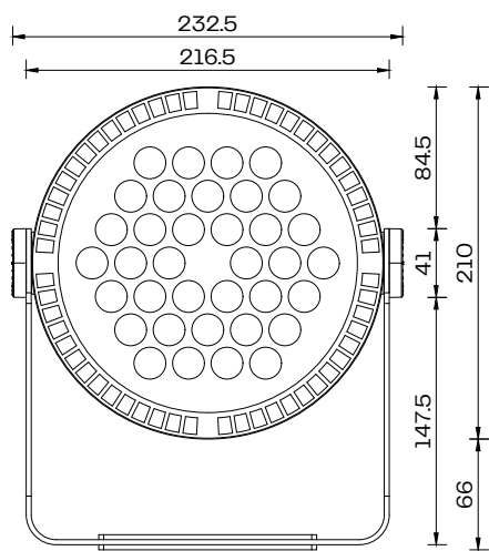
Beam F72 Front Scale 1:5
