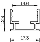
Mounting Profile 1
