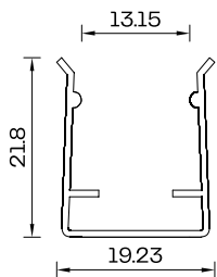
Profile Cross Section Flex Profile Scale 1:1
