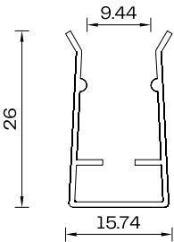
Profile Cross Section Flex Profile Scale 1:1
