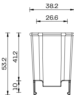
Top Head Scale 1:2
