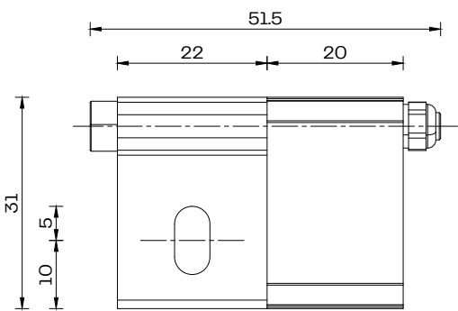
Angle Mounting Clip Scale 1:1
