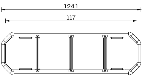
Top Head Scale 1:2
