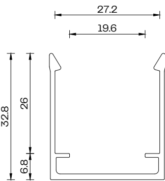
Mounting Clip Scale 1:1
