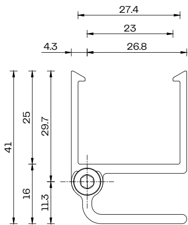
Angle Mounting Clip Scale 1:1
