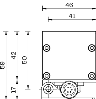
Linear Window Surface Mount Scale 1:2
