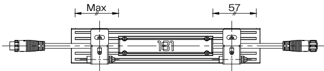
Linear Window Surface Mount Scale 1:5
