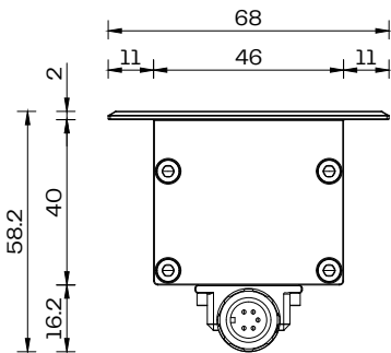
Linear Window Recessed Scale 1:2
