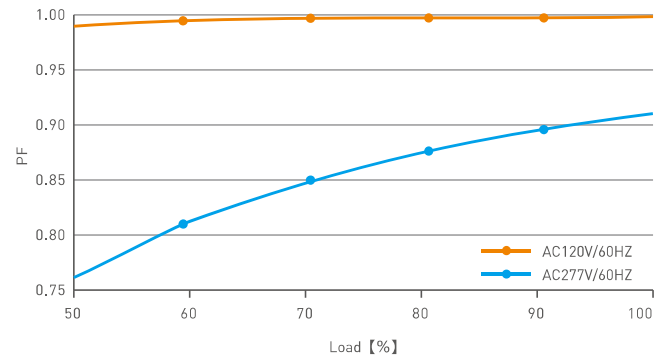
Power Factor Characteristic
