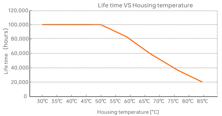
LM-150-12-G1M2F
