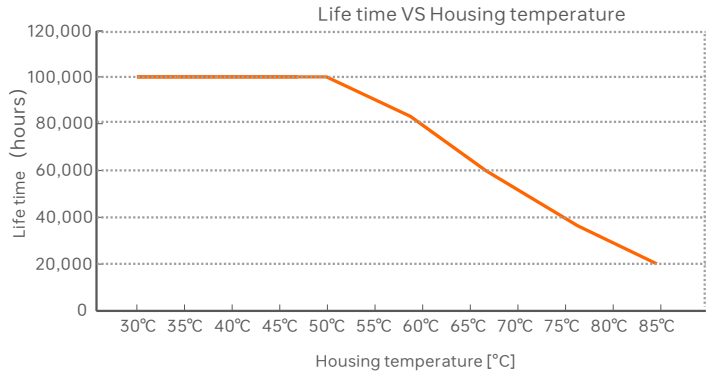
LM-150-24-G1M2F
