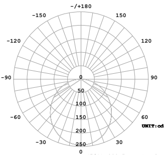
1121 - 111.5° Average Beam Angle
