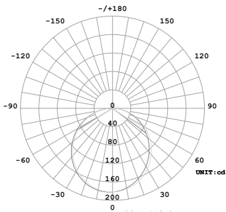
1010 - 112.8° Average Beam Angle
