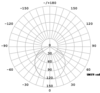
0816 - 113.1° Average Beam Angle
