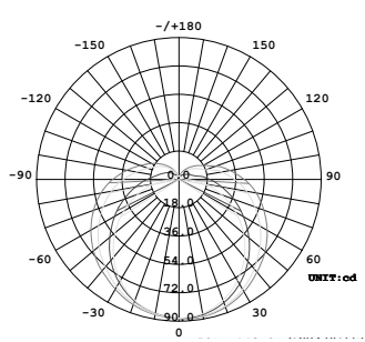
1128 - 143.2° Average Beam Angle
