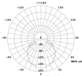
1616 - 113.5° Average Beam Angle
