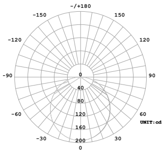
1313 - 113.5° Average Beam Angle
