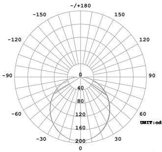
2219 - 112.7° Average Beam Angle
