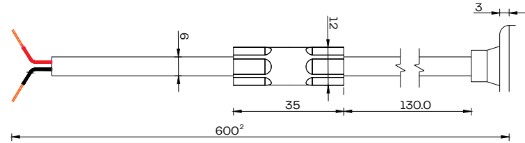
Single Color Bare Wires with waterstop 1
