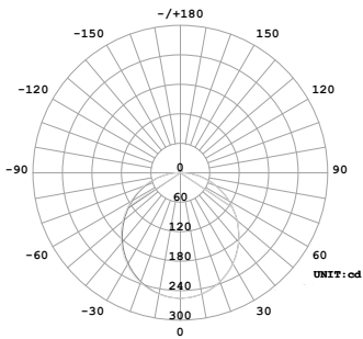
1010 - 112.9° Average Beam Angle
