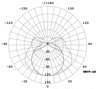
1717 - 158.9° Average Beam Angle
