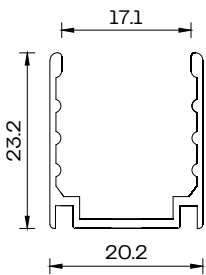
Profile Cross Section Curved Profile Scale 1:1
