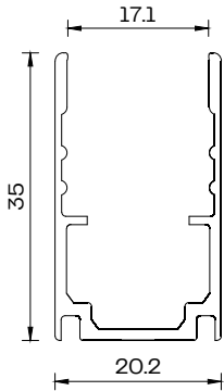
Profile Cross Section Cable Duct Profile Scale 1:1
