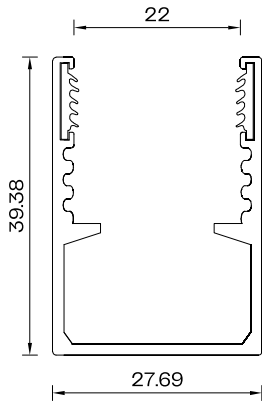
Profile Cross Section Curved Profile Cable Duct Scale 1:1
