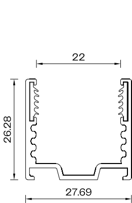
Profile Cross Section Side Bend Curved Profile Scale 1:1
