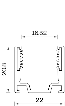
Profile Cross Section Curved Profile Scale 1:1
