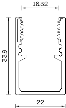
Profile Cross Section Curved Profile Cable Duct Scale 1:1
