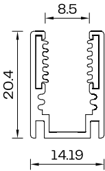
Profile Cross Section Curved Profile Scale 1:1
