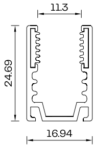
Profile Cross Section Curved Profile Scale 1:1
