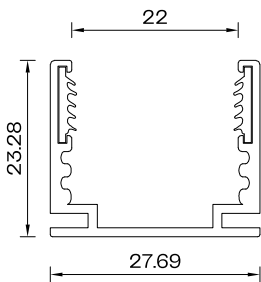
Profile Cross Section Straight Profile Scale 1:1
