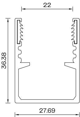
Profile Cross Section Cable Duct Profile Scale 1:1
