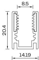
Profile Cross Section Straight Profile Scale 1:1
