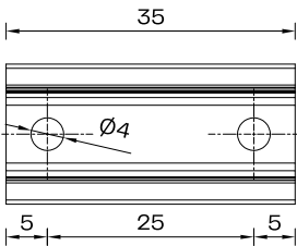
Mounting Clip Scale 1:1
