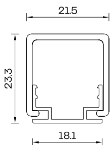
Profile Cross Section Straight Profile Scale 1:1
