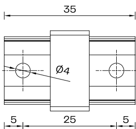
Mounting Clip Scale 1:1
