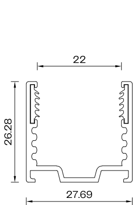
Profile Cross Section Straight Profile Scale 1:1
