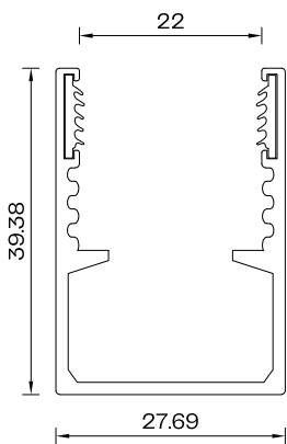
Profile Cross Section Cable Duct Profile Scale 1:1
