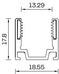
Profile Cross Section Curved Profile Scale 1:1
