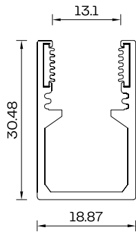
Profile Cross Section Curved Profile Cable Duct Scale 1:1
