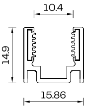
Profile Cross Section Curved Profile Scale 1:1
