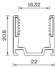
Profile Cross Section Curved Profile Scale 1:1
