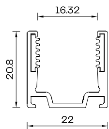
Profile Cross Section Curved Profile Scale 1:1
