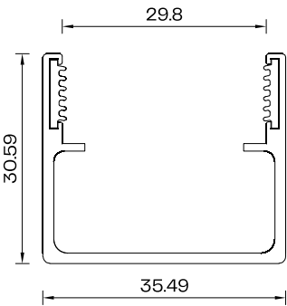
Profile Cross Section Curved Profile Scale 1:1
