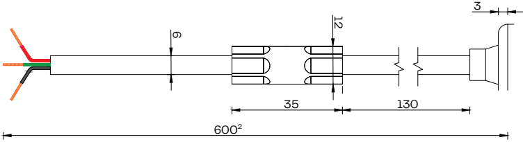
SPI Bare Wires with waterstop 1
